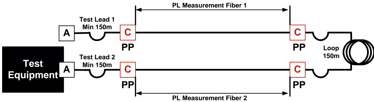
OTDR Loop measurement B to A
