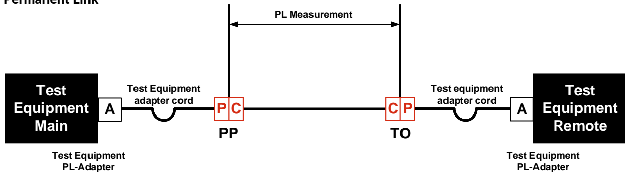
Sample test link PL
