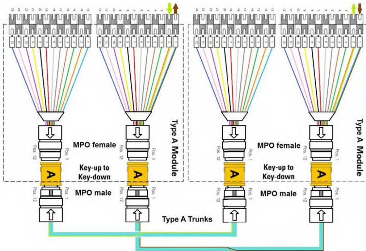
MPO polarity method A fan-out
