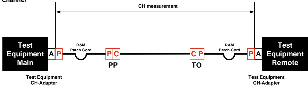
Sample test link CH
