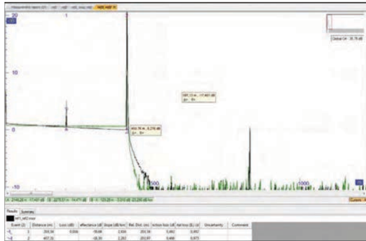
Test lead 1&2 reference connector verification
