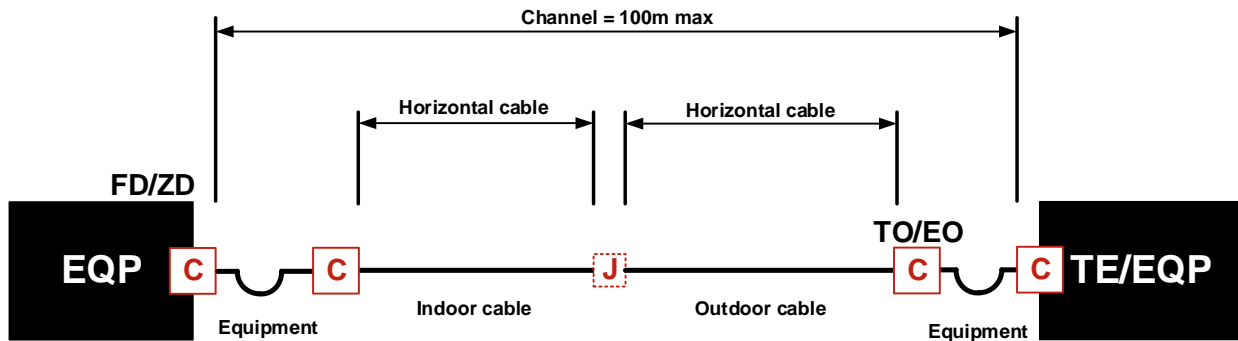
Coupled PL Indoor/Outdoor MPTL with Cable Coupler
