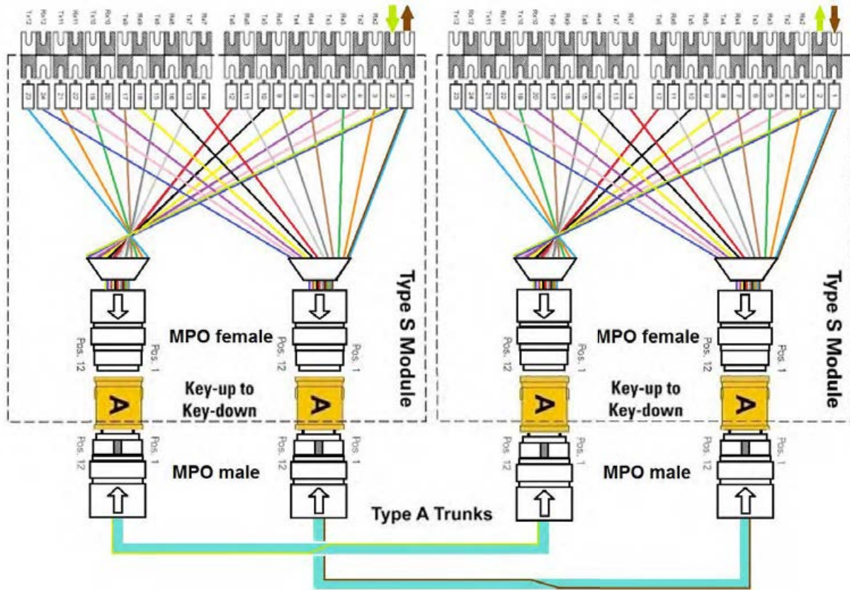
MPO polarity method with R&M fan-out Trunk A
