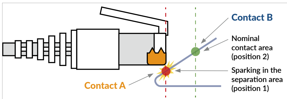
Spark when disconnection under load
