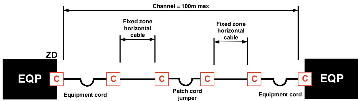
BtB interconnect model
