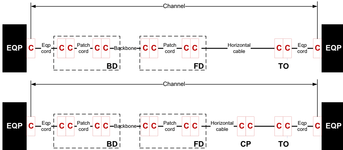
FO 5 connector direct combined
