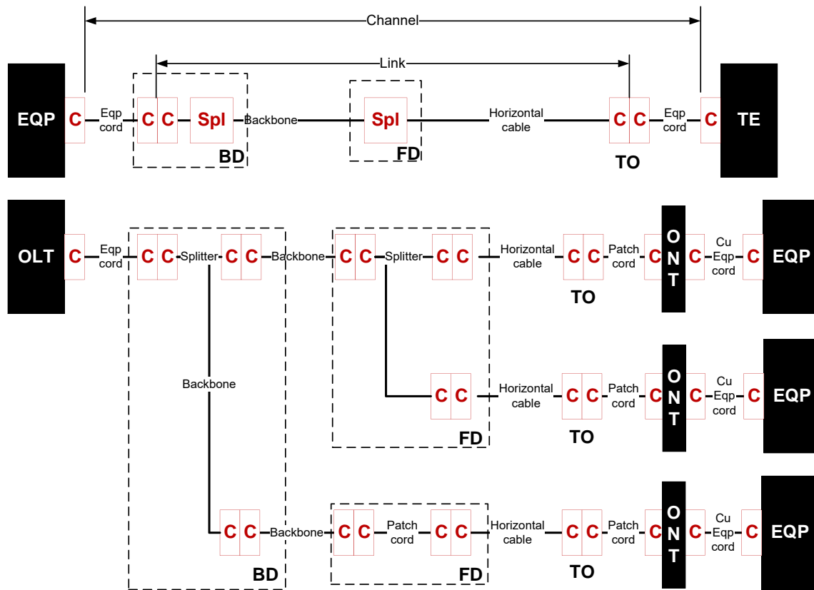
POLAN sample configuration
