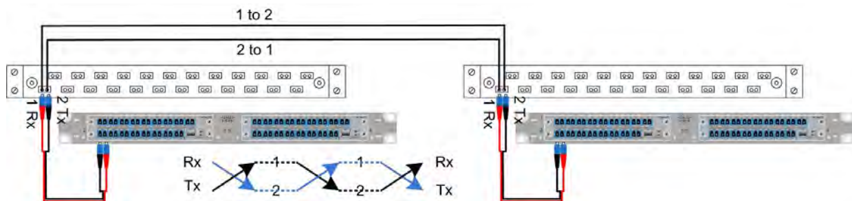
FO crossed backbone polarity
