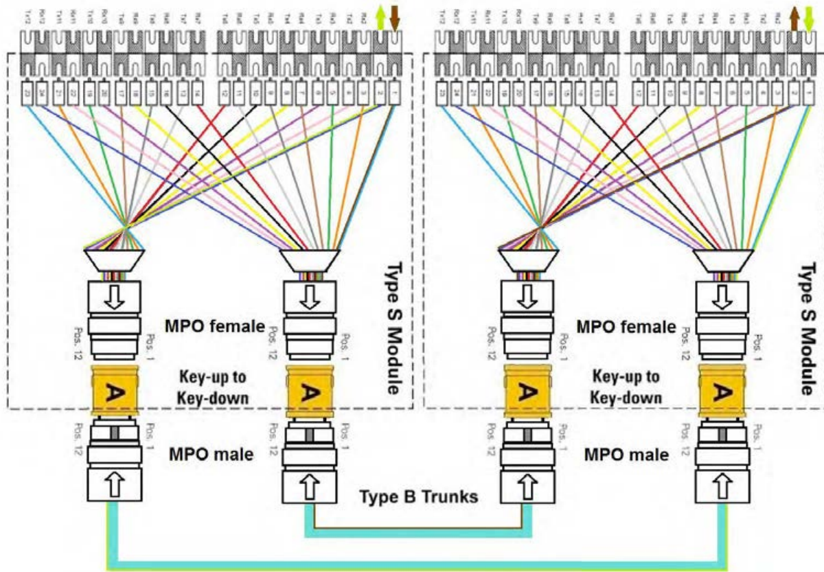
MPO polarity method with R&M fan-out Trunk B
