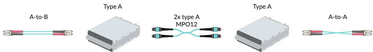
MPO polarity method A components
