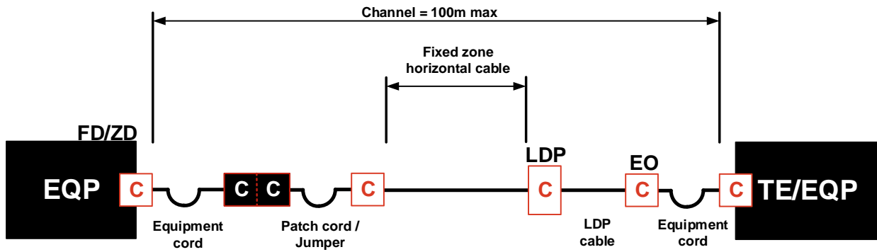
Cross connect LDP EO model with RJ45 Coupler
