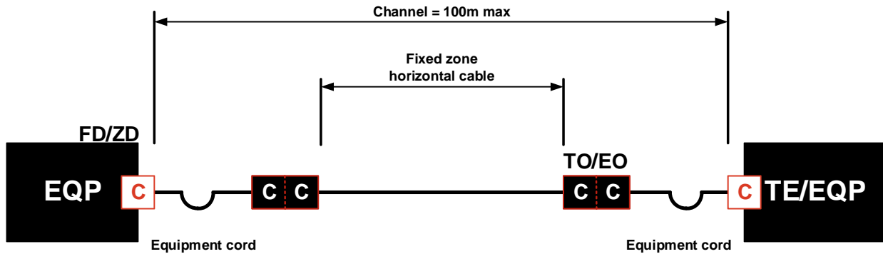
Interconnect TO/EO model with RJ45 Coupler
