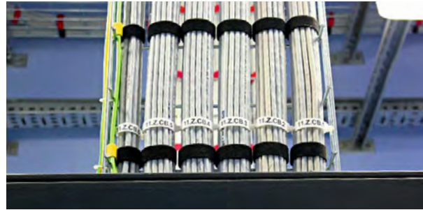
Correct fastening of vertical cables
