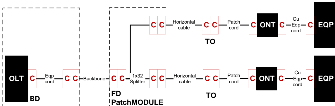
POLAN calculation sample
