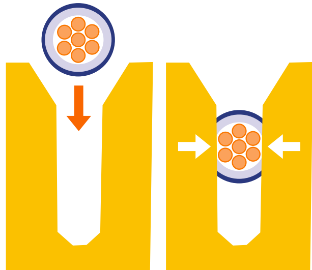
IDC contact
