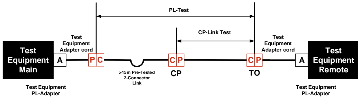
Sample test link PL with CP Method 2
