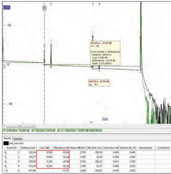
Unidirectional loop measurement
