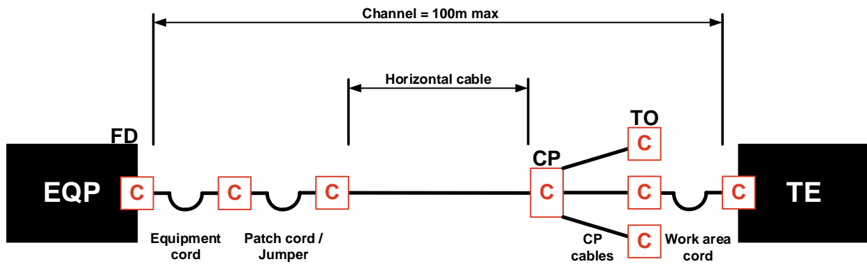
Cross connect-CP-TP model
