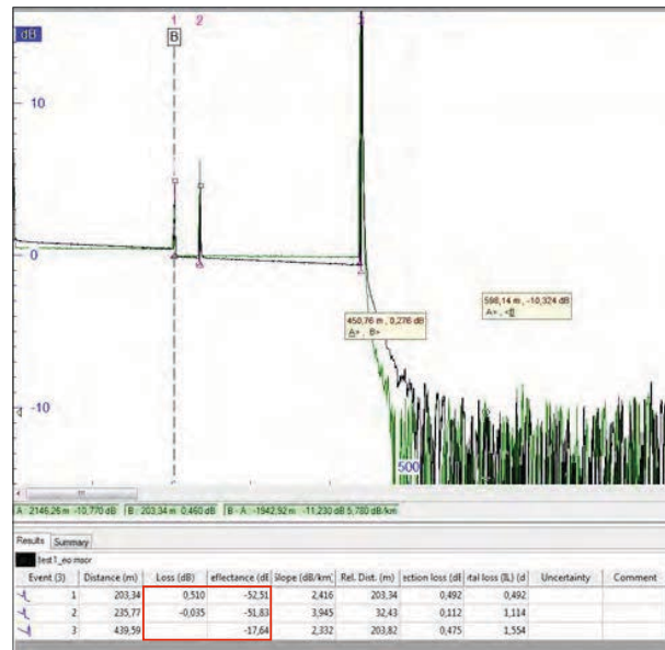
MMF measurement origin to end
