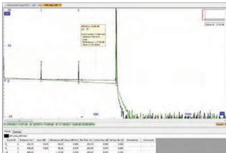
Test leads and loop reference connector verification
