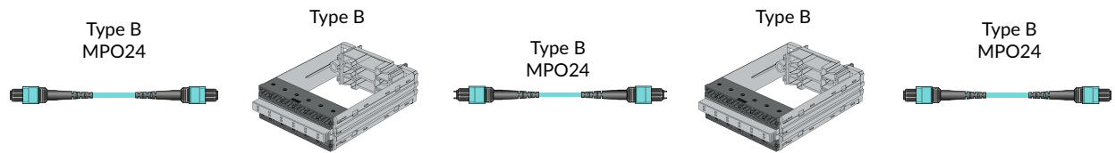
MPO polarity method R&M 40/100G Trunk B
