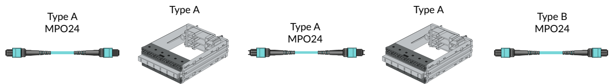
MPO polarity method R&M 40/100G Trunk A
