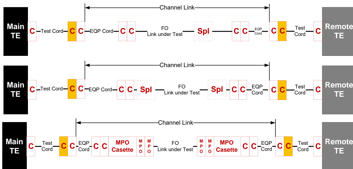
FO Channel test configuration
