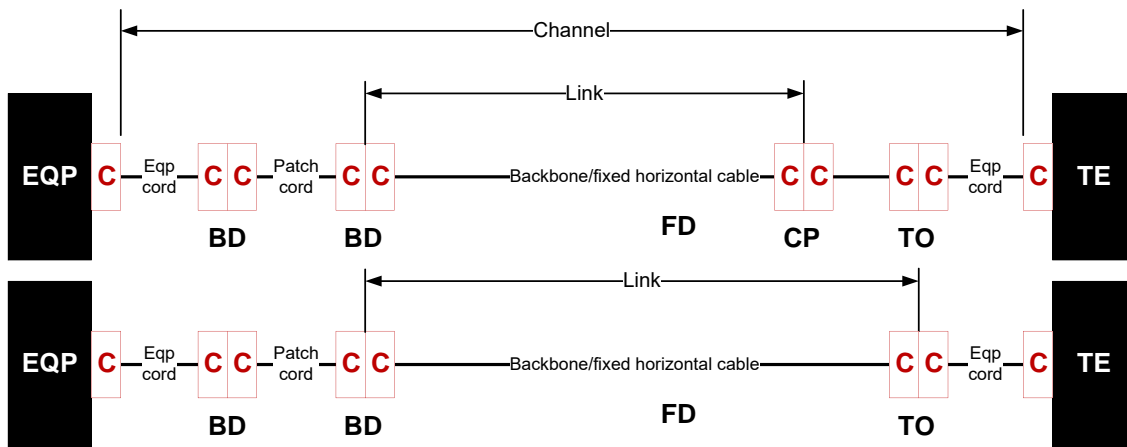
FO 3 Connector direct combined
