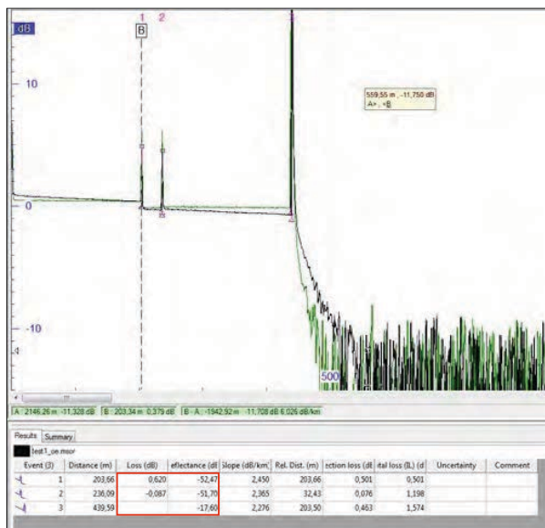
MMF measurement end to origin
