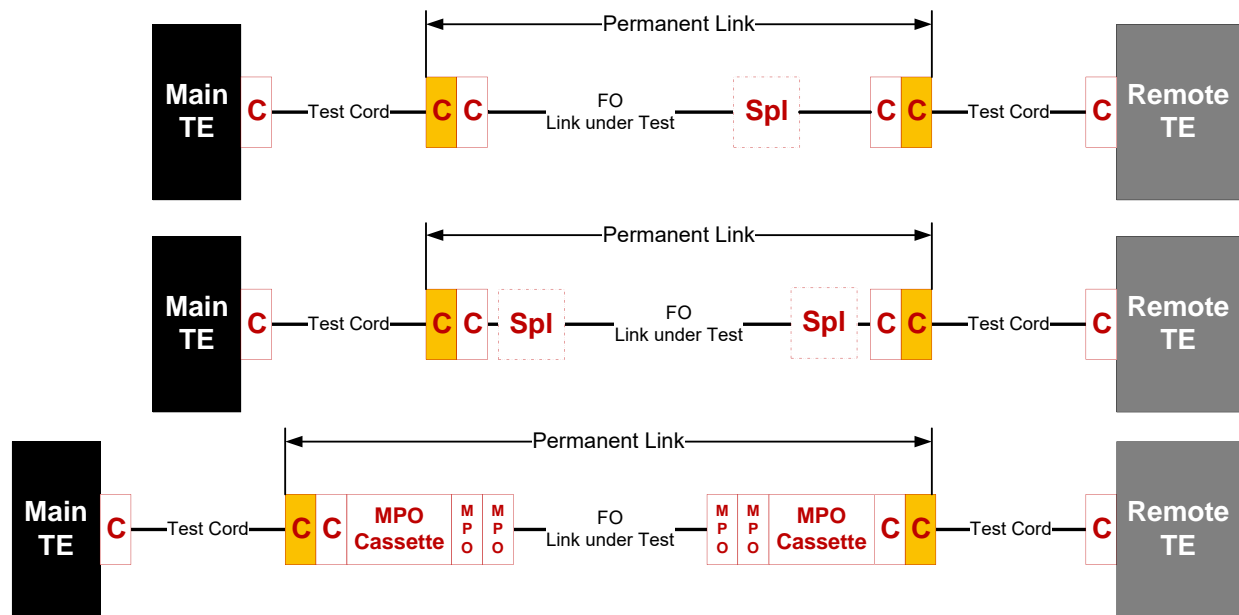
FO Cabling Permanent Link Configuration
