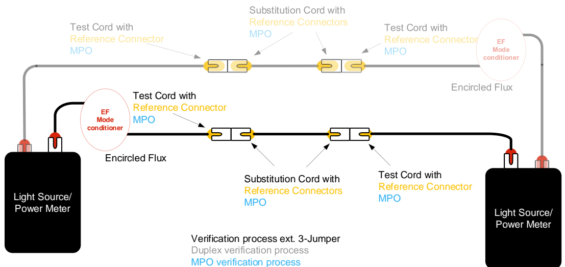
«extended 3-Jumper» method verification
