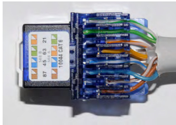
Incorrect wiring
