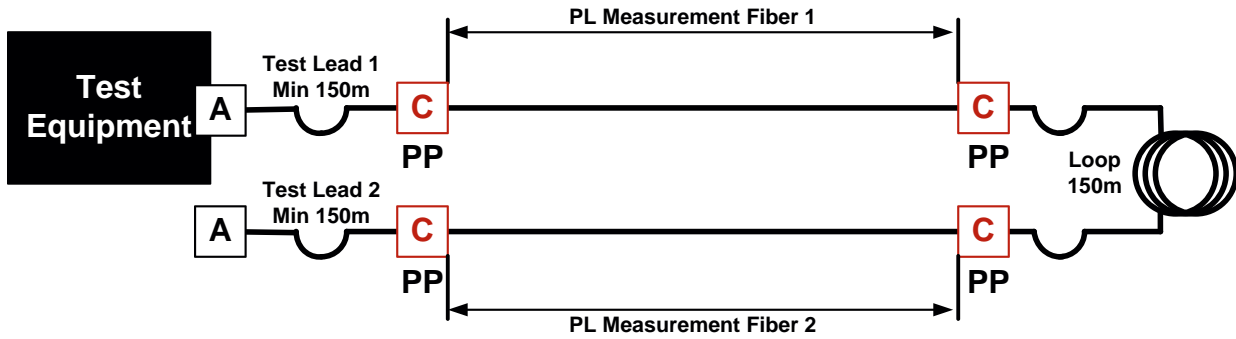
OTDR Loop measurement A to B
