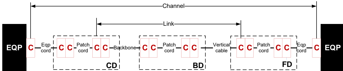
FO sample calculation LAN
