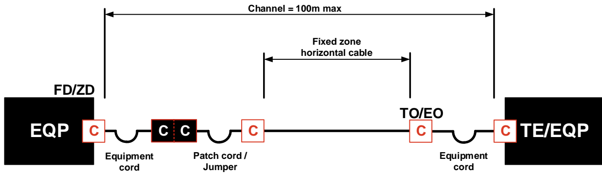
Cross connect TO/EO model with RJ45 Coupler
