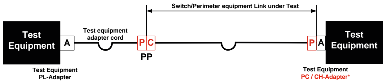
Sample test link MPTL
