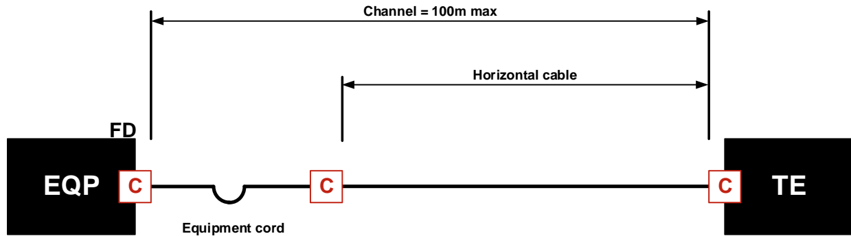
LAN one connector model
