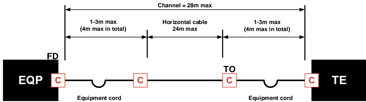
Schematic representation of Cat. 8.1 channel with length specification
