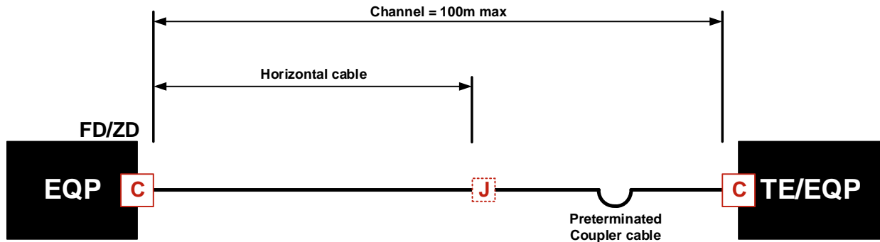
OC/DC 1-Connector Model MPTL with Cable-Coupler
