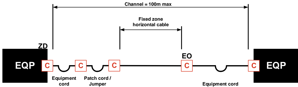
Cross connect-EO model
