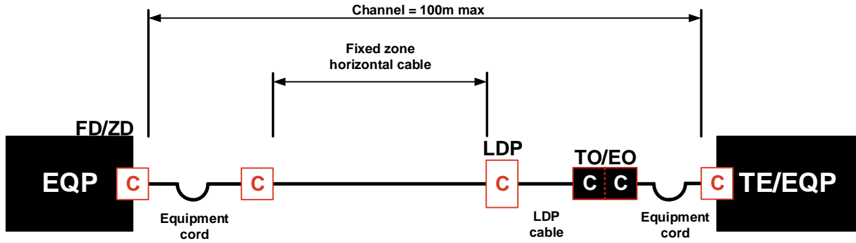
Interconnect LDP EO model with RJ45 Coupler
