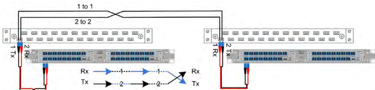
FO straight backbone polarity
