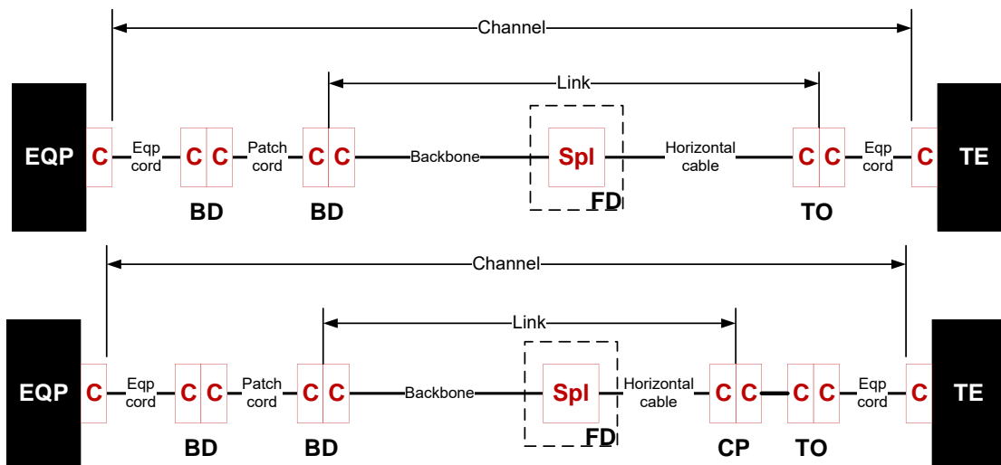
FO 4 connector combined splice
