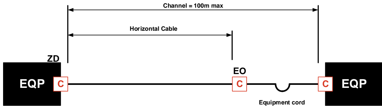
DC one connector model
