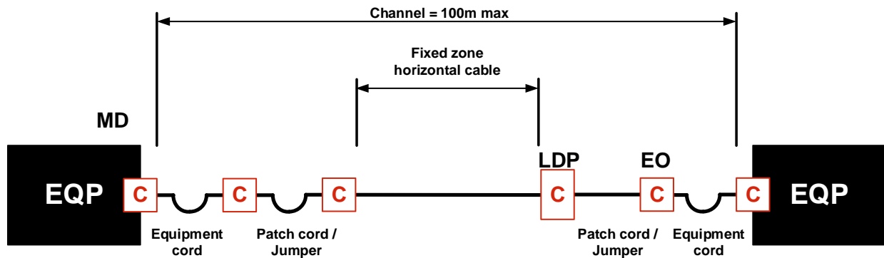
Main Distributor channel model
