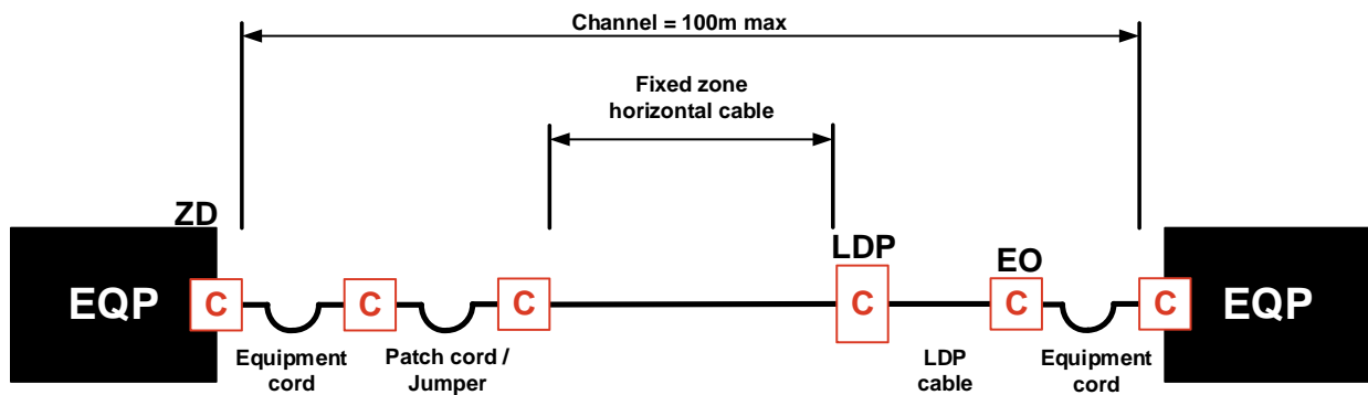
Cross connect-LDP-EO model
