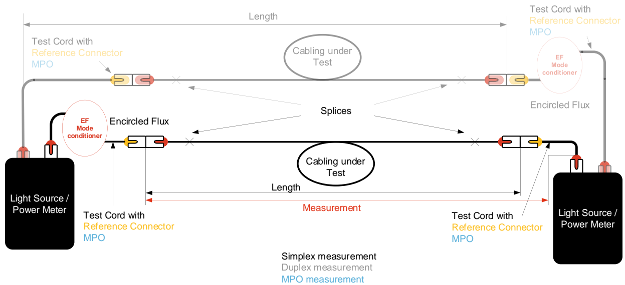
Measurement of a PL
