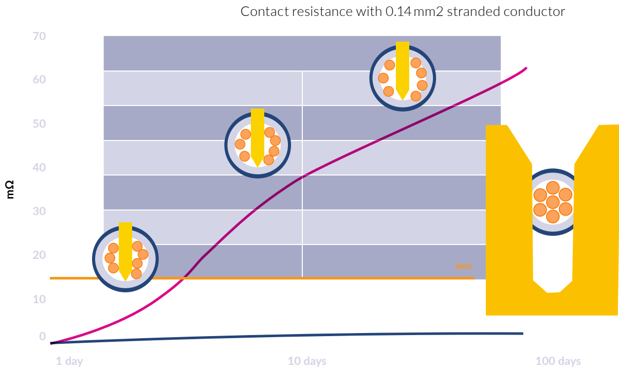
Resistance behavior
