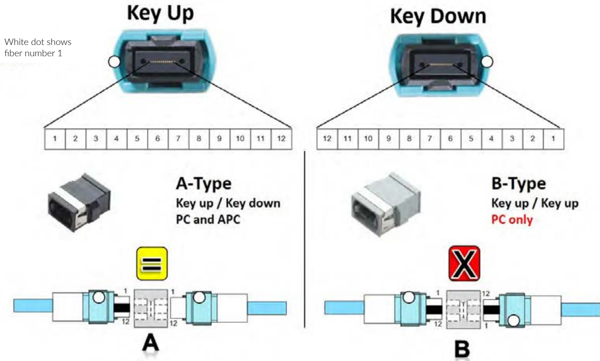
Key Up and Key Down
