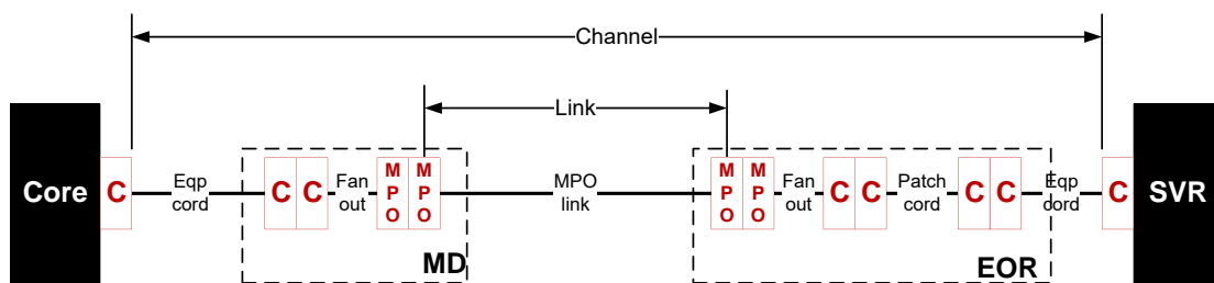
FO sample Calculation DC
