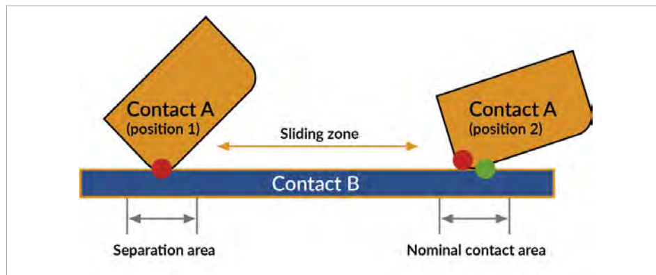
Displacement contact point during plugging process
