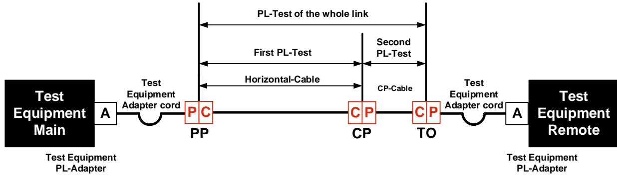
Sample test link PL with CP Method 1
