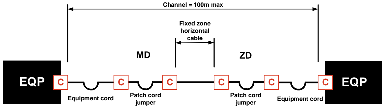
Cross-inter-cross connection model
